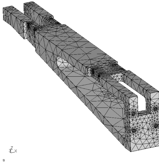
Figure 12: CAD-geometry meshed with tet-elements
