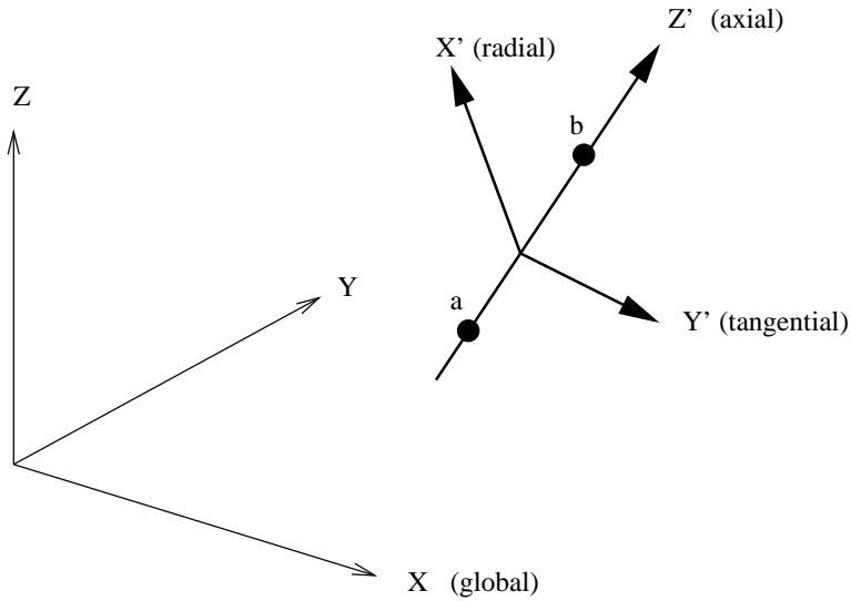
Figure 153: Definition of a cylindrical coordinate system
