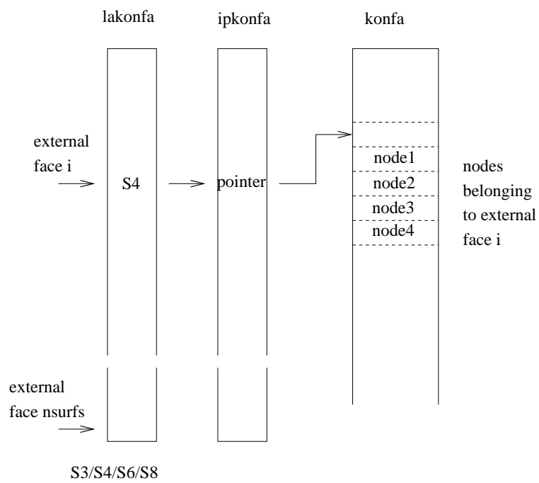
Figure 176: Data structure storing the kind of external face and the nodes belonging to that face
