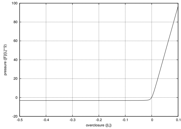
Figure 129: Linear pressure-overclosure relationship
