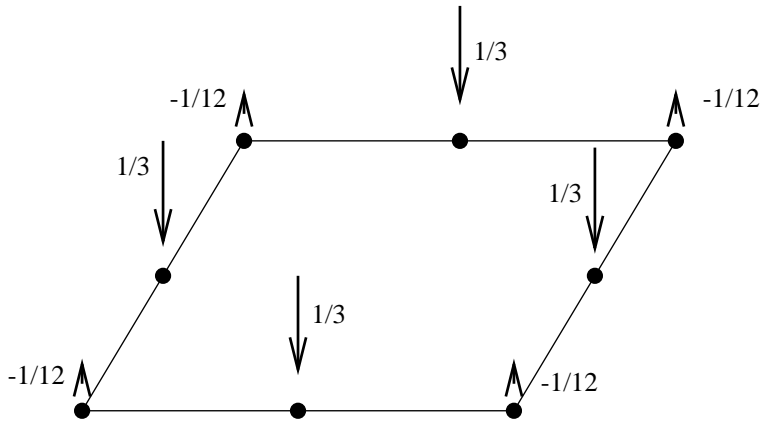
Figure 145: Equivalent nodal forces for a face of a C3D20(R) element
