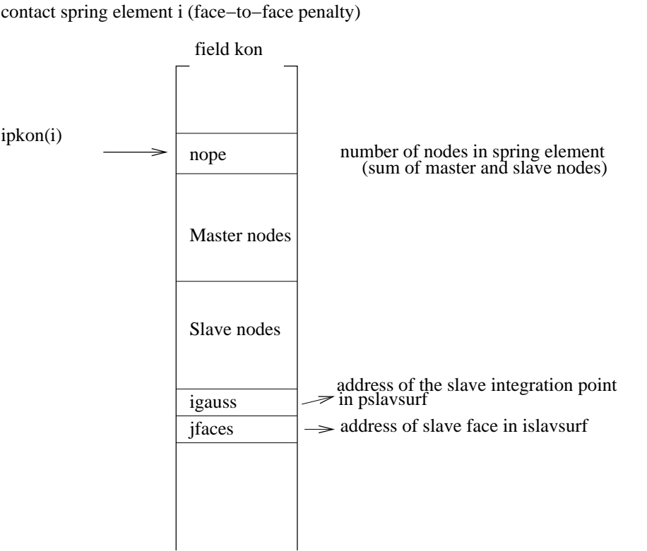
Figure 169: Topology of the face-to-face penalty contact elements
