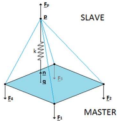
Figure 127: Creation of a node-to-face penalty contact element
