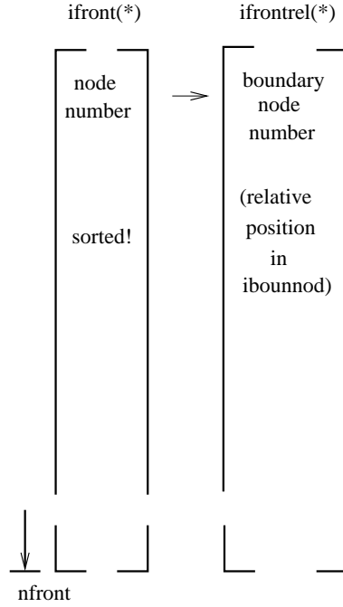
Figure 189: Fields for the front nodes (before analyzing the adjacency relations)
