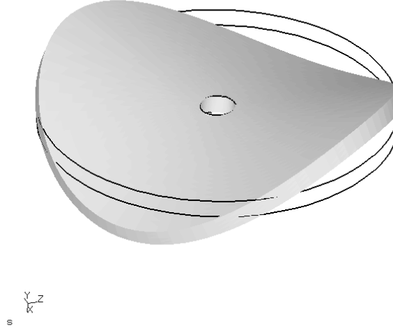
Figure 135: Eigenmode for a full disk with a nodal diameter of two
