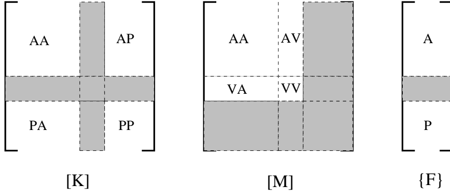
Figure 140: Nonzero parts of the governing matrices
