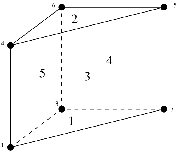
Figure 144: Face numbering for wedge elements
