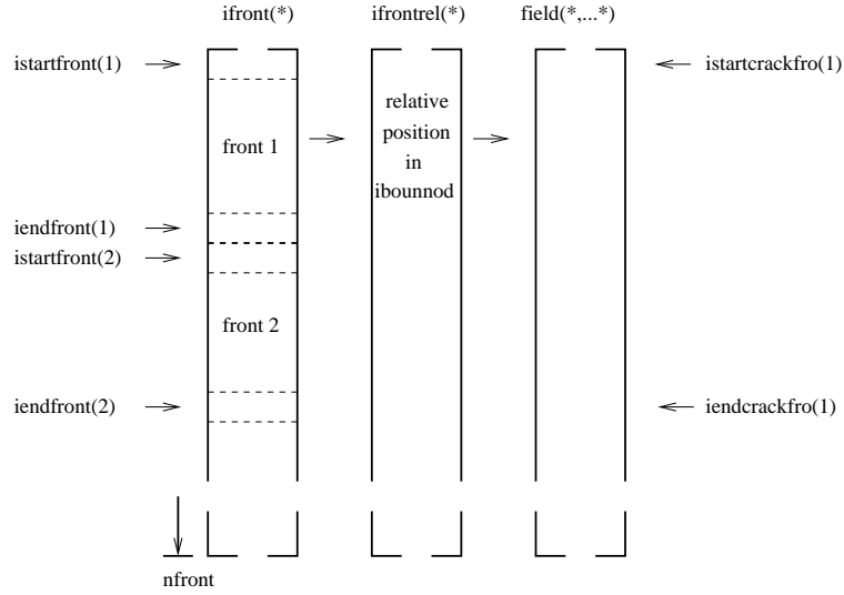
Figure 190: Fields for the front nodes (after analyzing the adjacency relations)
