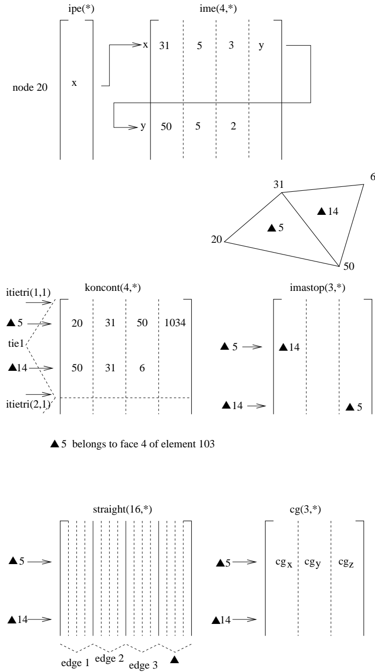
Figure 161: Storage of the triangulation properties
