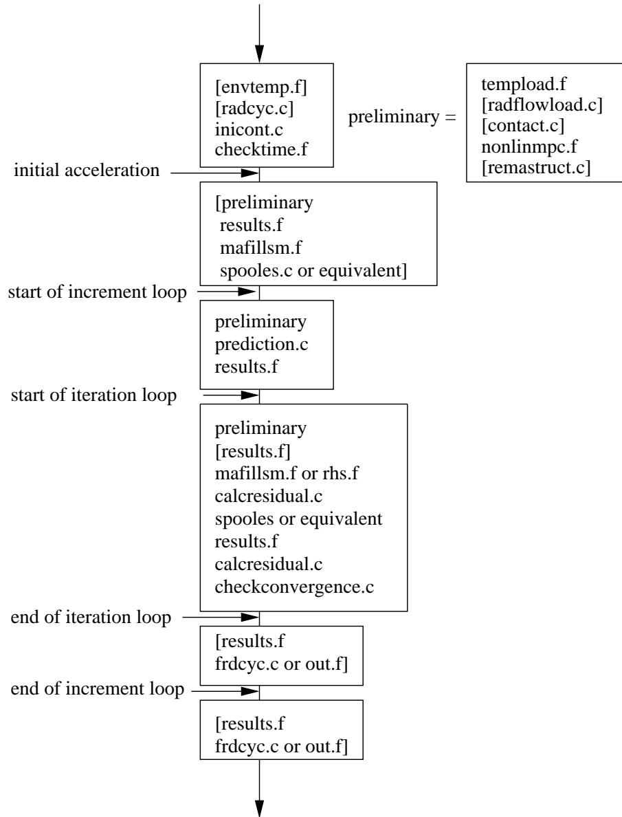
Figure 170: Flow diagram for subroutine nonlingeo
