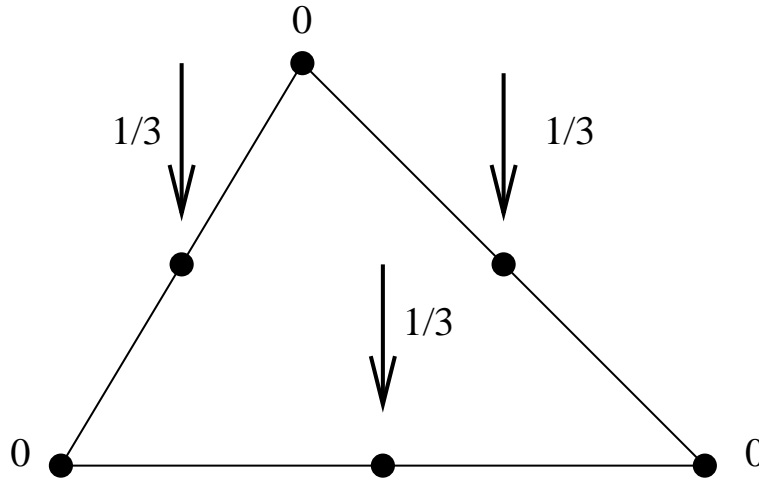
Figure 146: Equivalent nodal forces for a face of a C3D10 element
