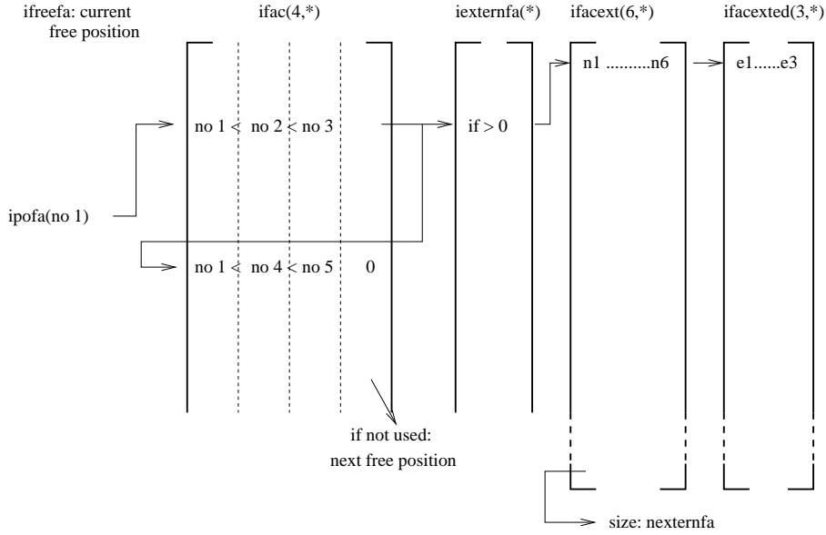
Figure 183: Node per face relationship
