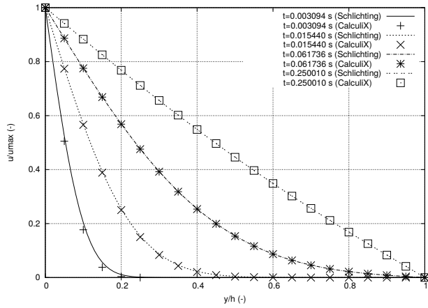
Figure 28: Velocity across the space in between the plates for different times
