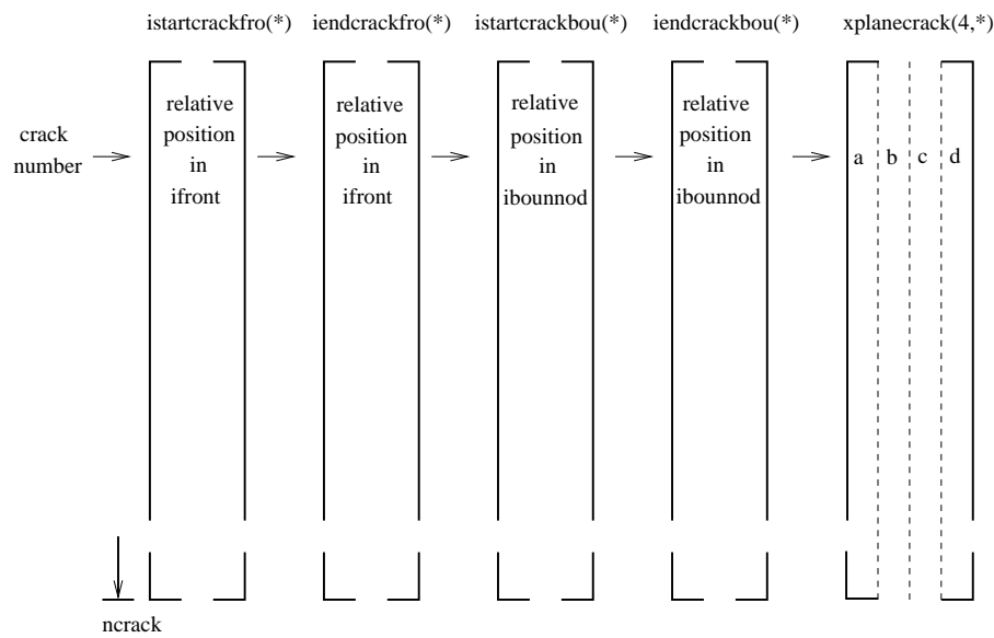
Figure 192: Fields for the crack characteristics
