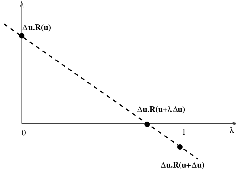
Figure 141: Principle of the line search method
