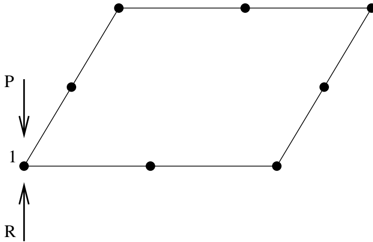
Figure 147: Point load in a node belonging to a 8-noded face
