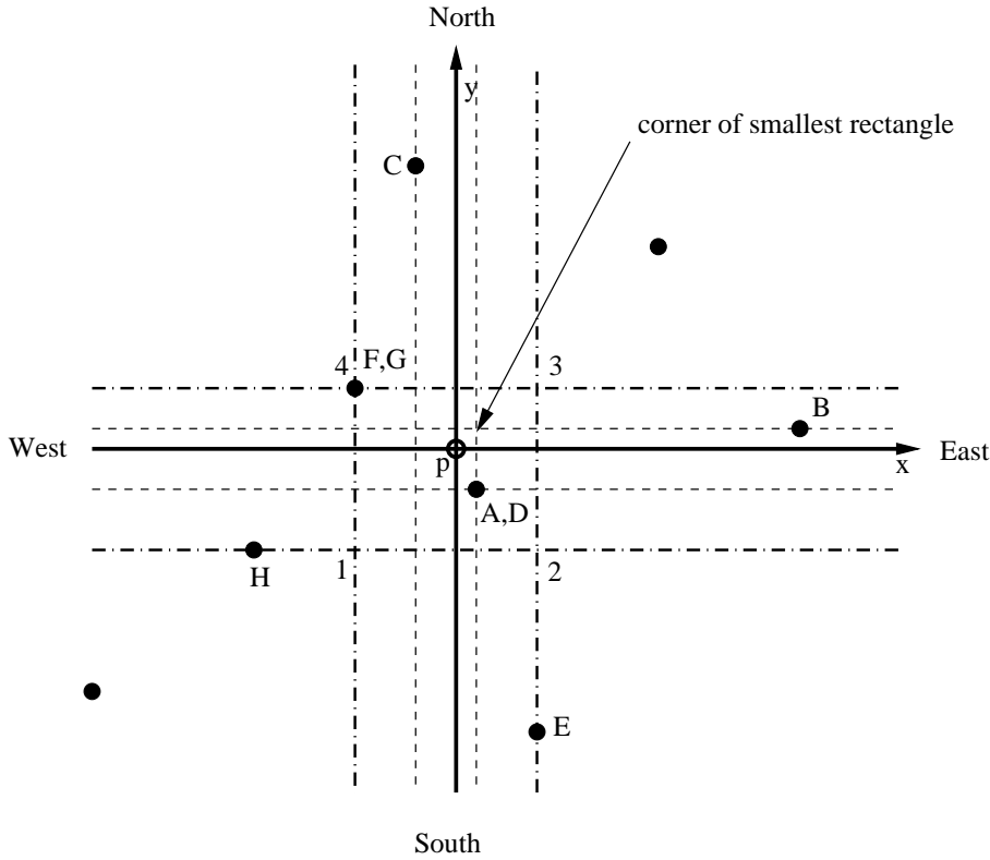
Figure 194: Scheme of the nearest point algorithm
