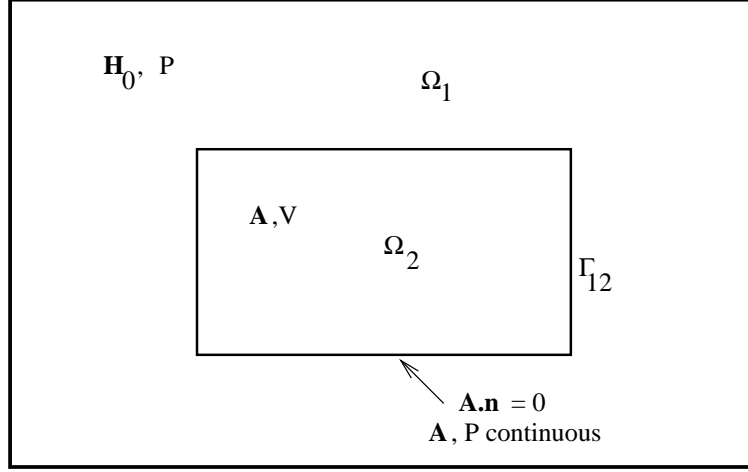
Figure 138: Electromagnetic setup for simply connected bodies
