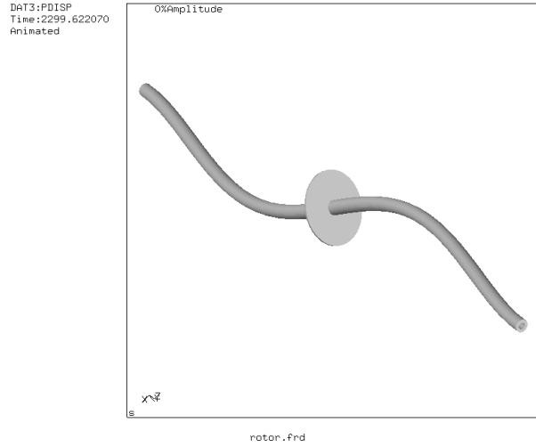
Figure 13: Three-node eigenmode
