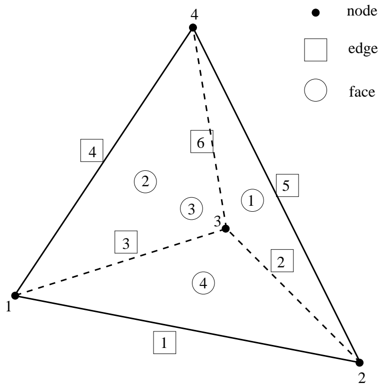
Figure 184: Node, edge and face numbering within a tetrahedral element
