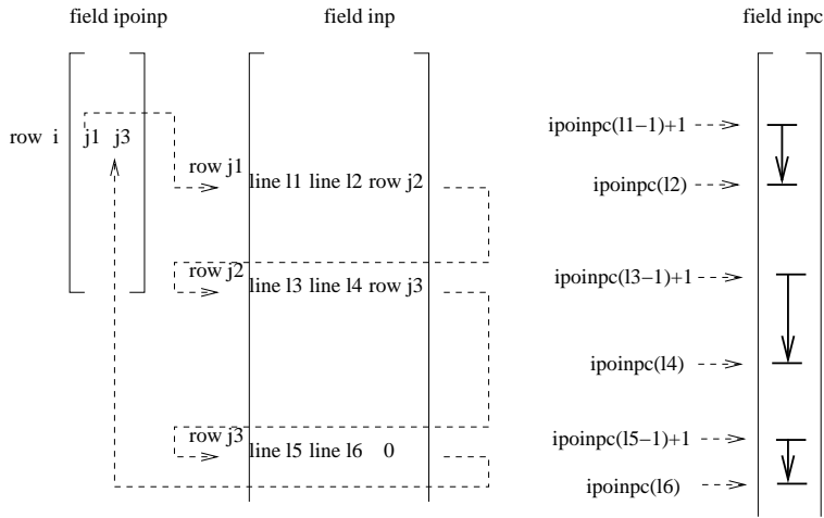
Figure 154: Reading the lines for keyword entry i
