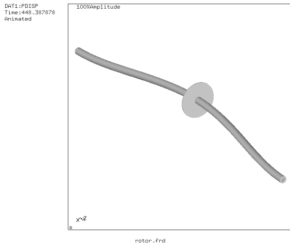
Figure 12: Two-node eigenmode
