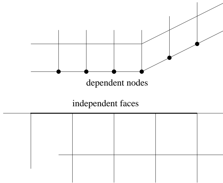
Figure 126: Definition of the dependent nodal surface and the independent element face surface
