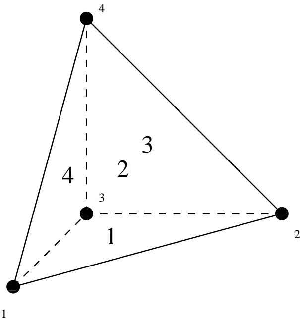
Figure 143: Face numbering for tetrahedral elements
