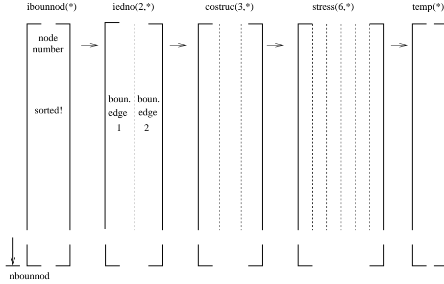
Figure 188: Fields for the boundary nodes and edges
