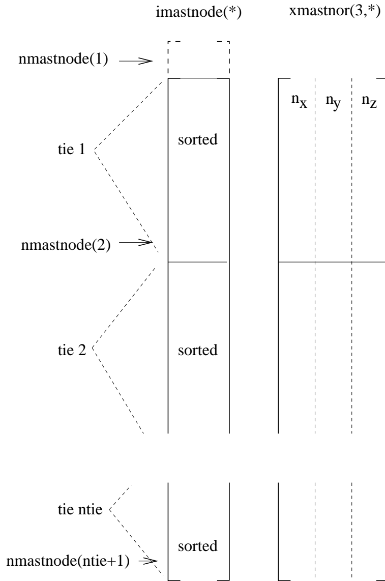
Figure 167: Storage of the master nodes
