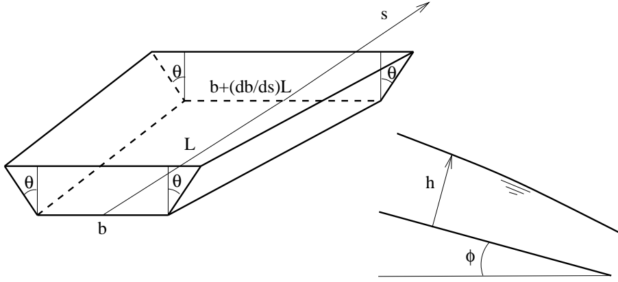
Figure 136: Channel geometry
