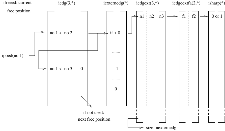
Figure 181: Node per edge relationship
