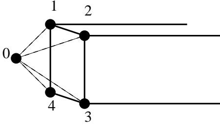
Figure 157: Beam element connection
