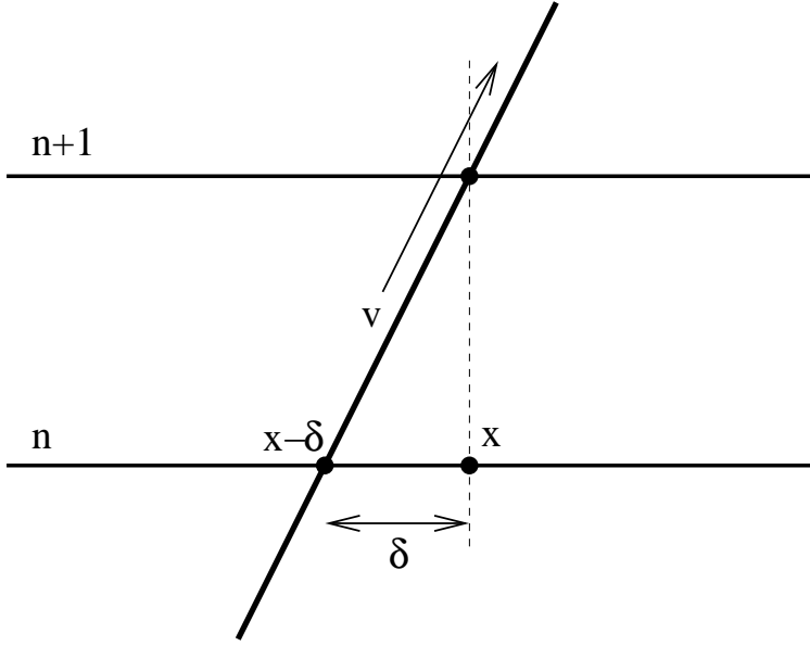
Figure 137: Formulating the equations along characteristics
