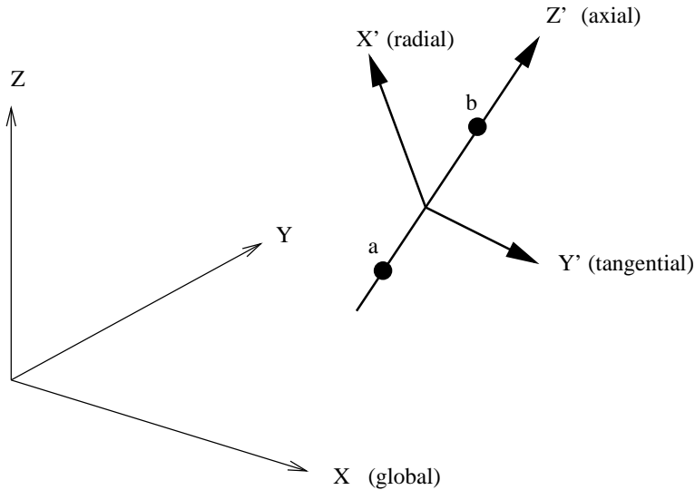
Figure 151: Definition of a cylindrical coordinate system
