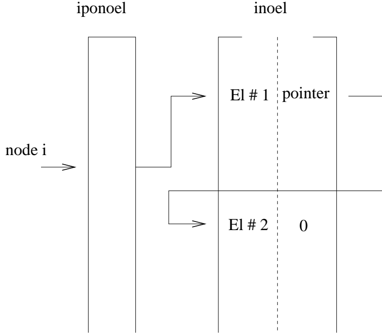
Figure 175: Data structure for all elements belonging to a given node
