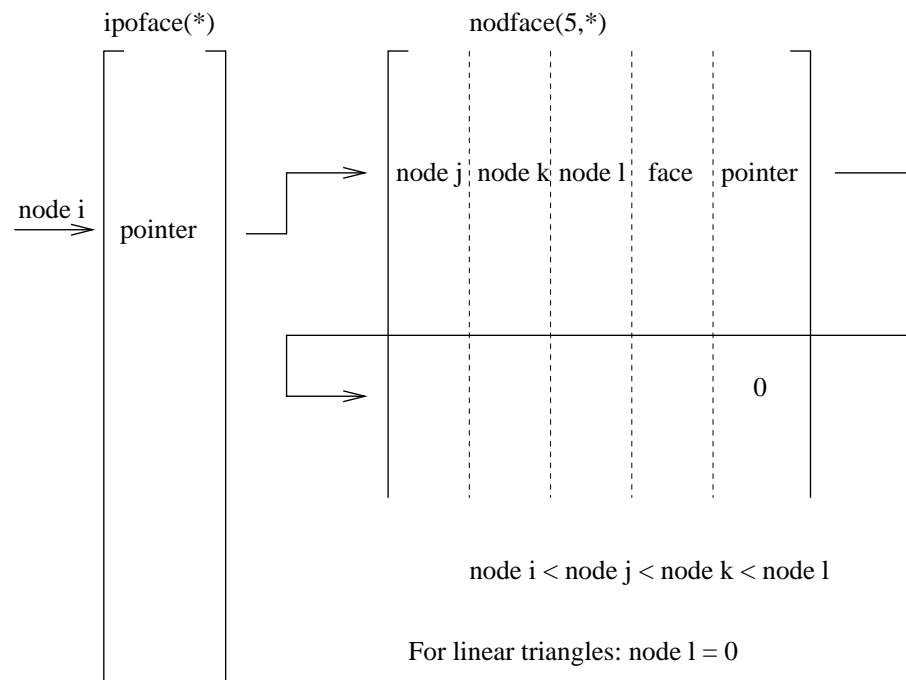
Figure 162: Storage of all faces for the determination of the external faces
