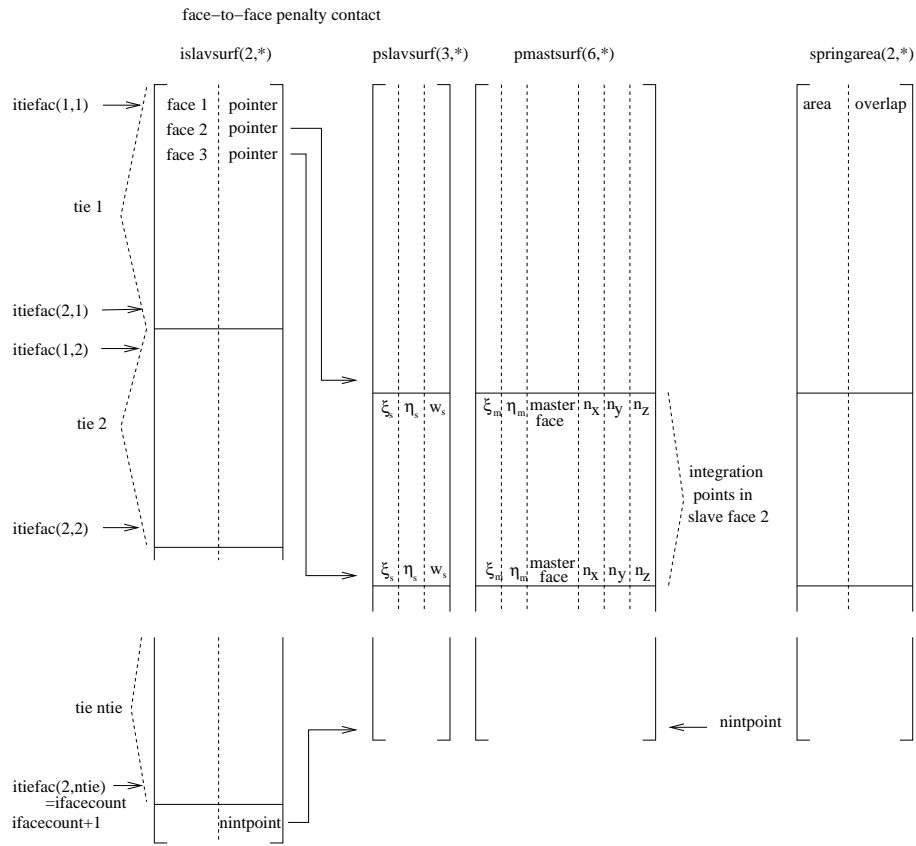
Figure 165: Storage of the slave faces (face-to-face penalty)
