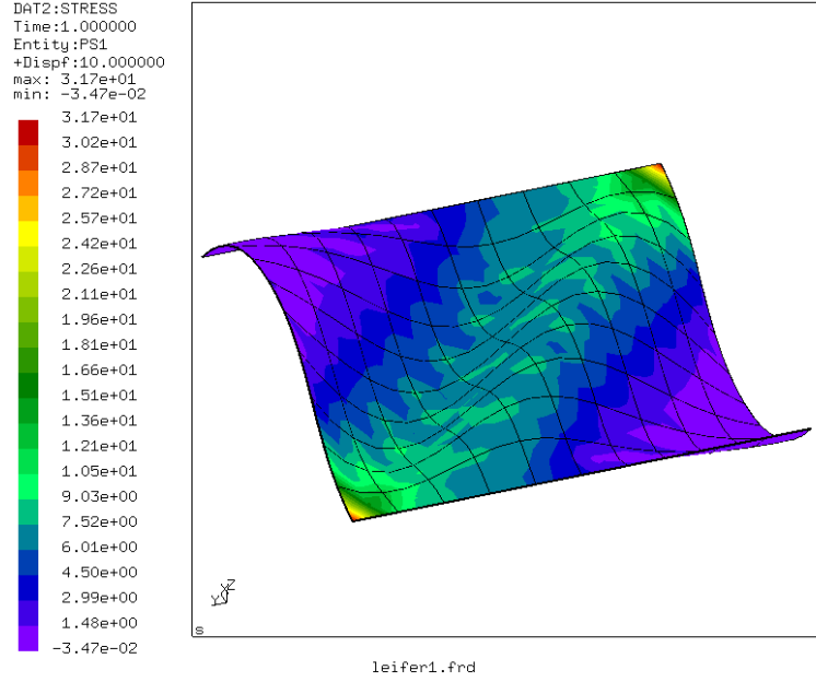
Figure 41: Maximum principal stress in the deformed sheet
