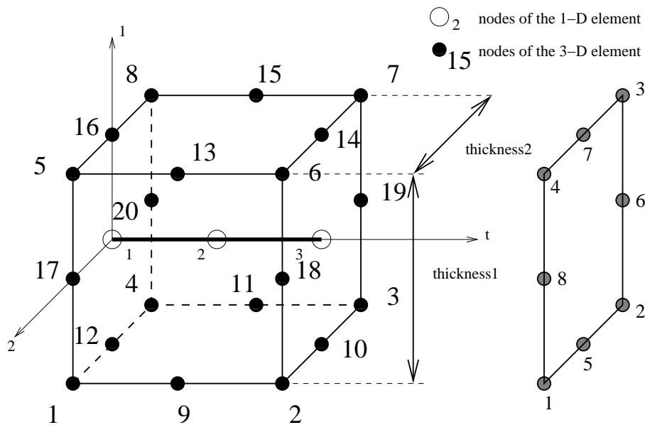
Figure 74: Expansion of a beam element
