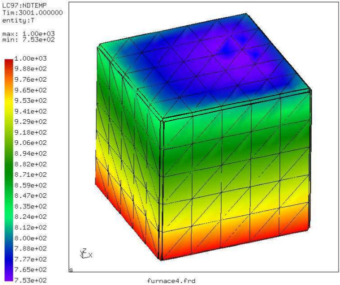
Figure 15: Temperature distribution at t=3001 s
