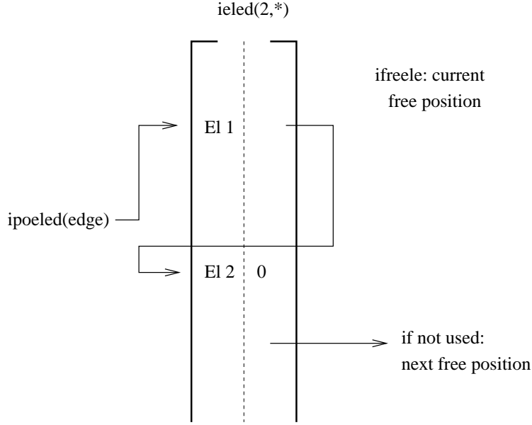
Figure 182: Element per edge relationship
