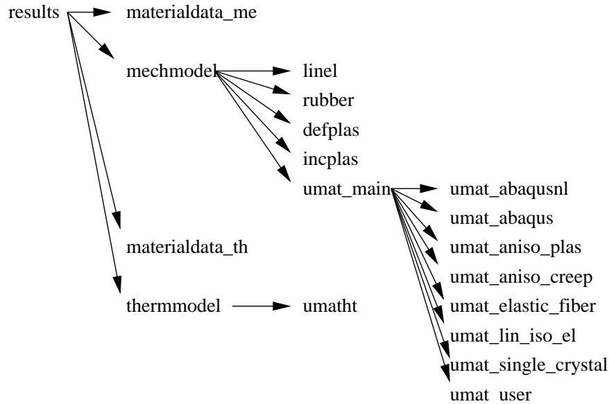
Figure 171: Flow diagram for subroutine results
