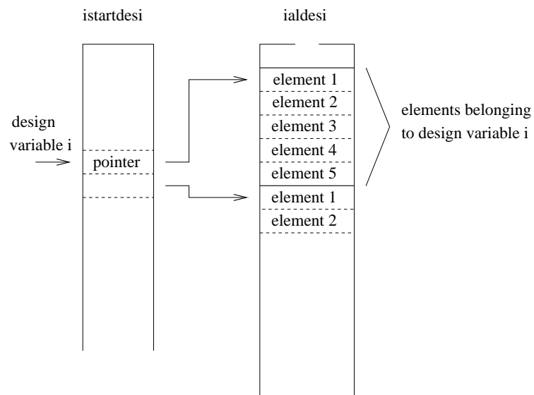
Figure 178: Data structure for all elements belonging to a specific design variable
