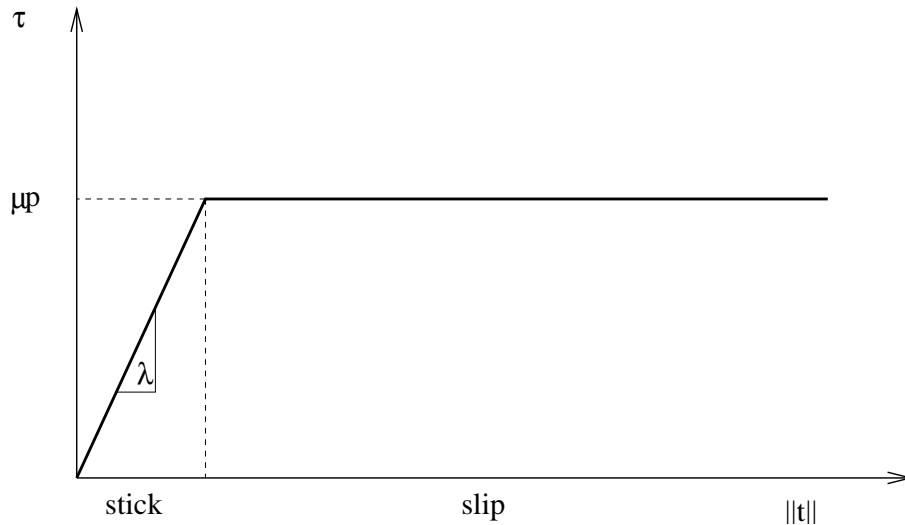
Figure 130: Shear stress versus relative tangential displacement
