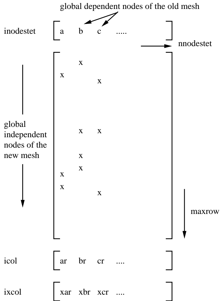
Figure 185: Matrix structure of the connecting equations
