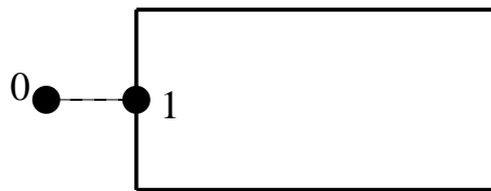
Figure 159: Plane and axisymmetric element connection
