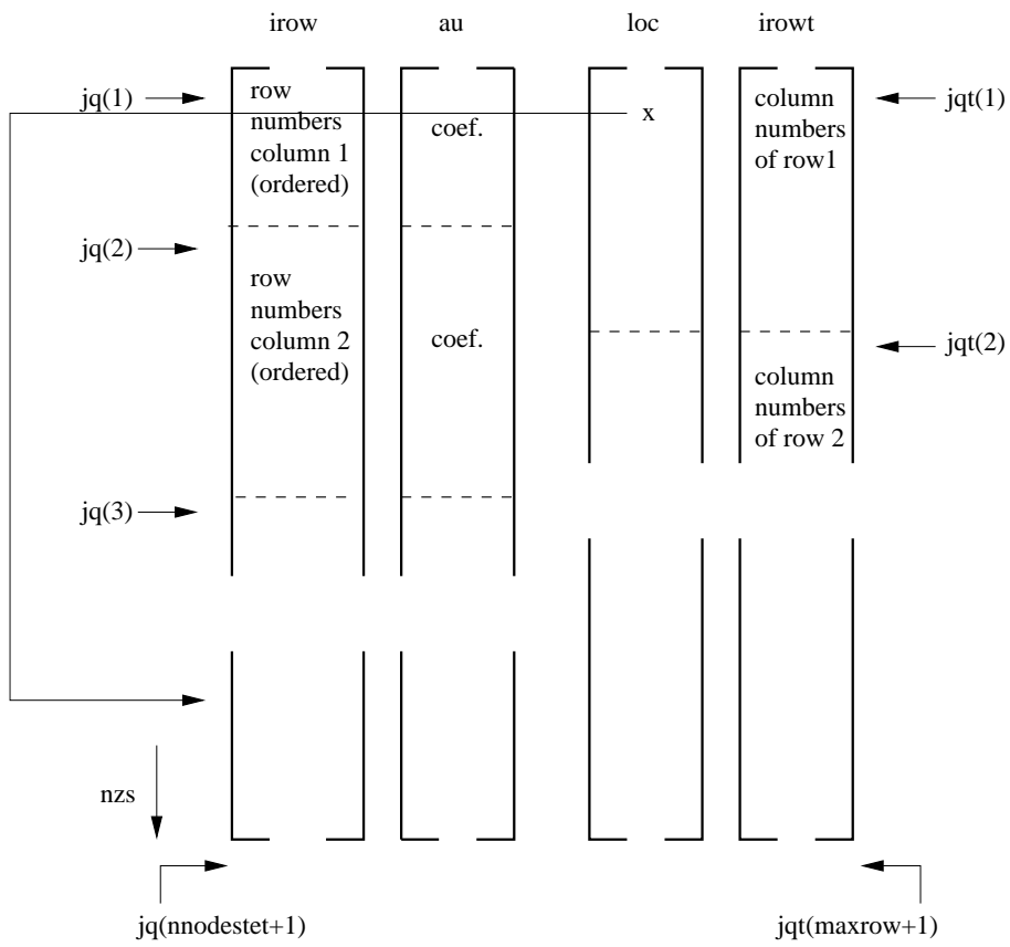
Figure 186: Fields describing the matrix structure
