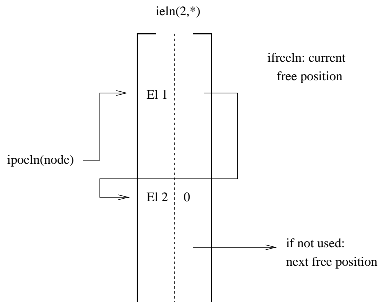
Figure 180: Element per node relationship
