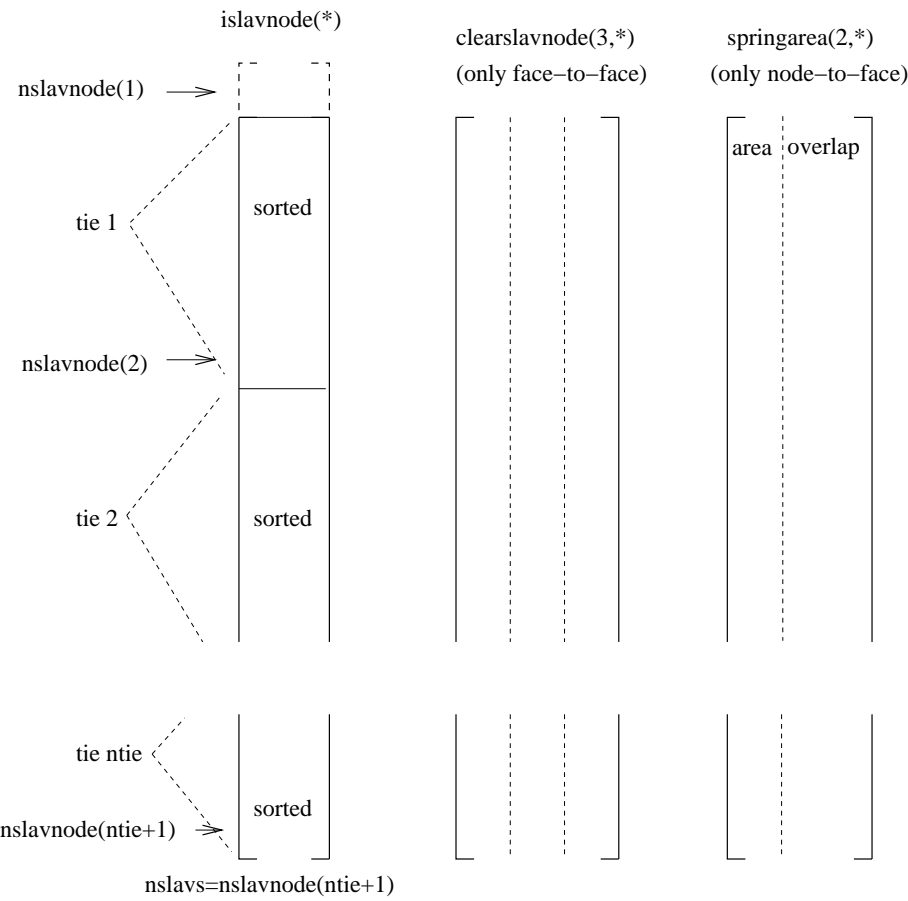
Figure 163: Storage of the slave nodes
