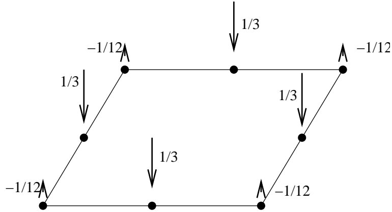
Figure 148: Equivalent forces of a uniform pressure on a plate (1 element)
