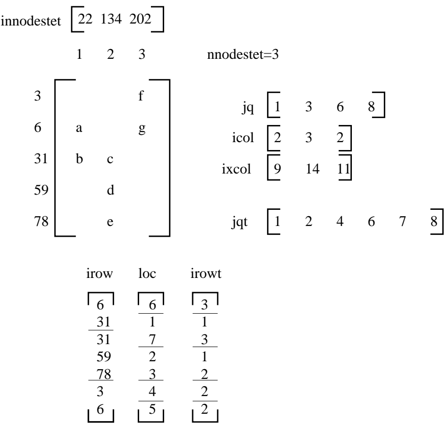
Figure 187: Example for the fields defining the connecting equations
