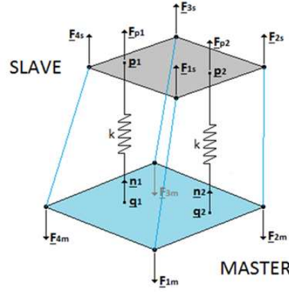
Figure 132: Creation of a face-to-face penalty contact element
