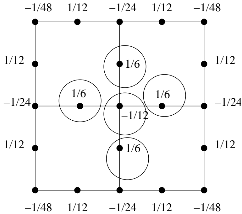
Figure 149: Equivalent forces of a uniform pressure on a plate (4 elements)
