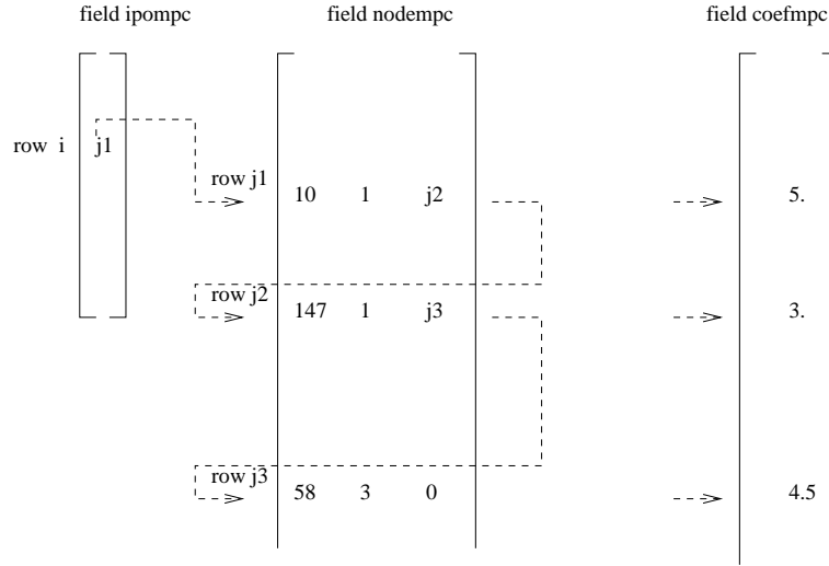
Figure 155: Example of the storage of a linear equation
