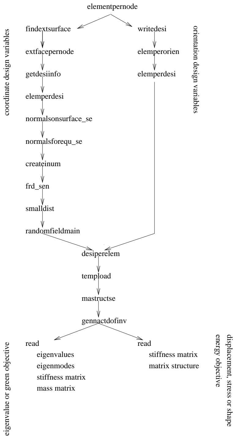
Figure 174: Structure of the preprocessing part
