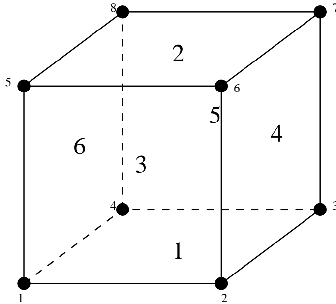
Figure 142: Face numbering for hexahedral elements
