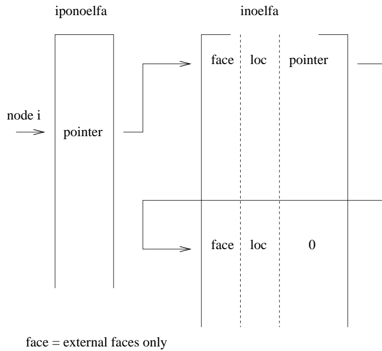
Figure 177: Data structure for all external faces belonging to a given node
