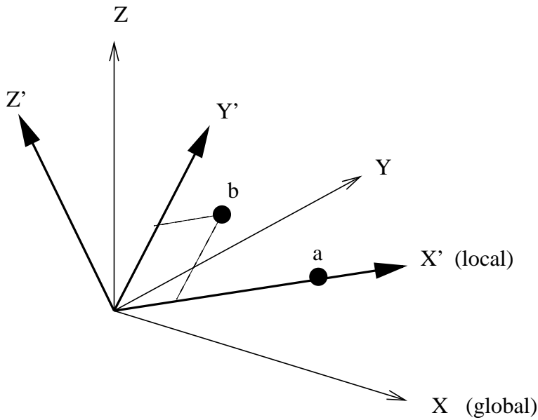
Figure 150: Definition of a rectangular coordinate system
