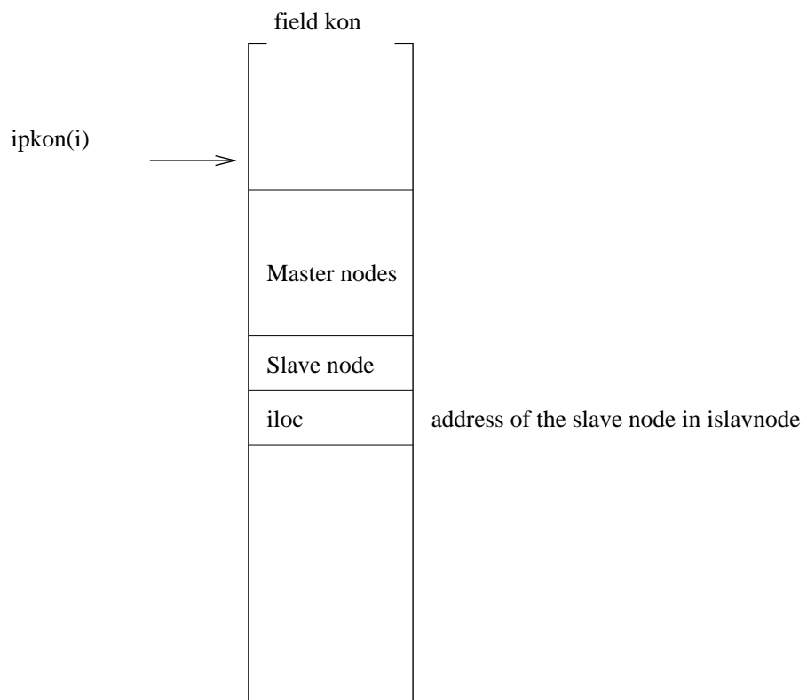
Figure 168: Topology of the node-to-face contact elemetns
