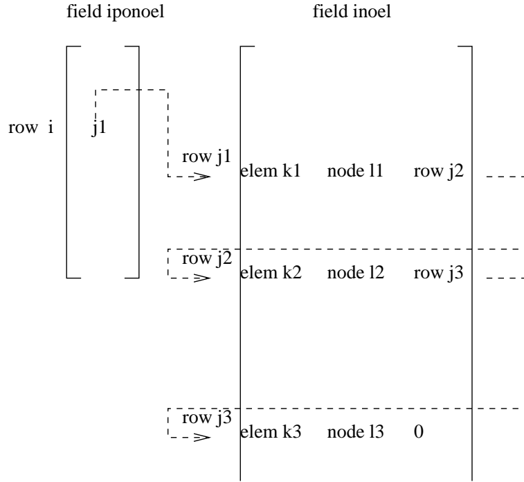
Figure 156: Structures to store all elements to which a given node belongs
