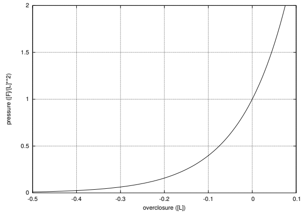
Figure 128: Exponential pressure-overclosure relationship
