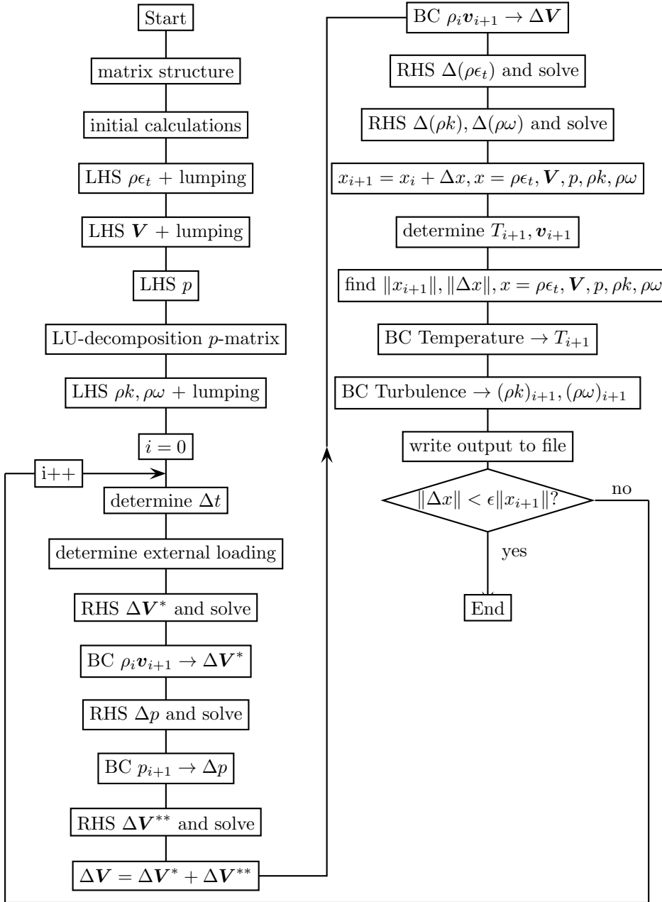
Figure 172: Flow diagram for liquids
