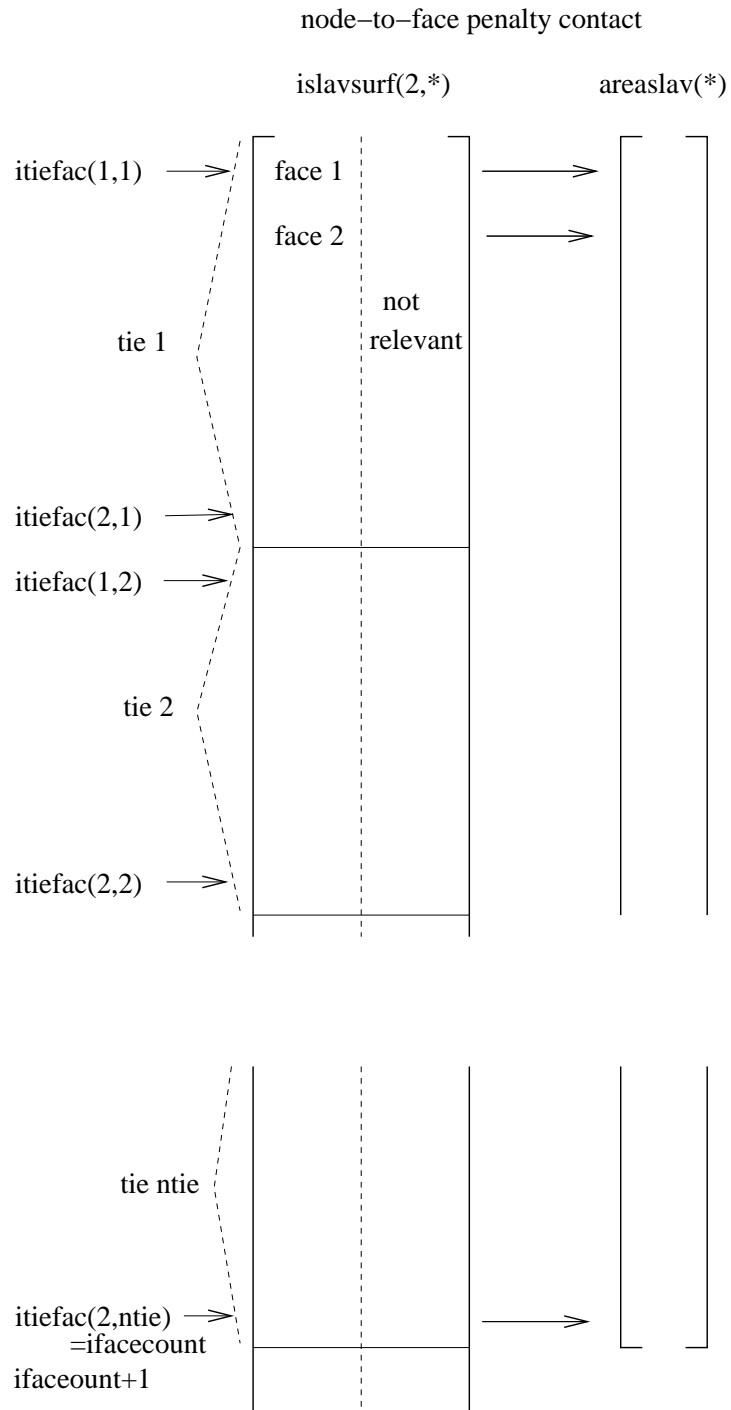
Figure 164: Storage of the slave faces (node-to-face penalty)
