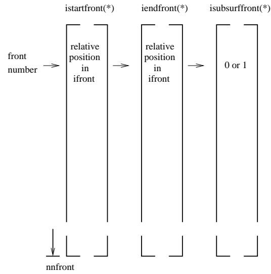
Figure 191: Fields for the front characteristics
