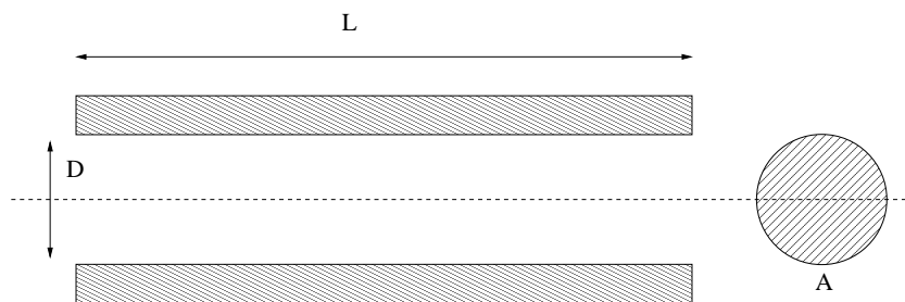
Figure 93: Geometry of the Gas Pipe element
