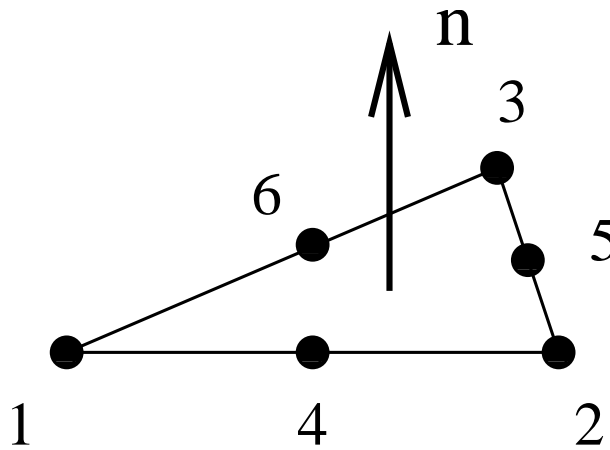
Figure 70: 6-node triangular element
