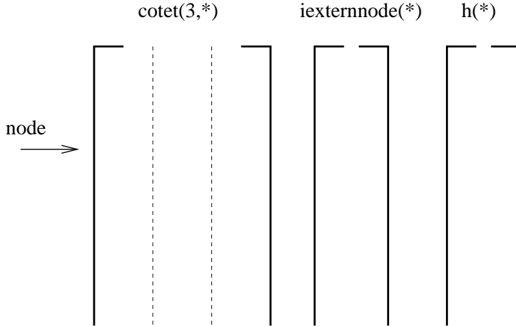
Figure 179: Nodal fields
