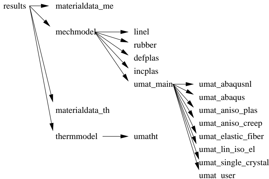
Figure 173: Flow diagram for subroutine results
