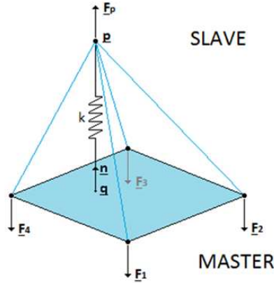
Figure 130: Creation of a node-to-face penalty contact element
