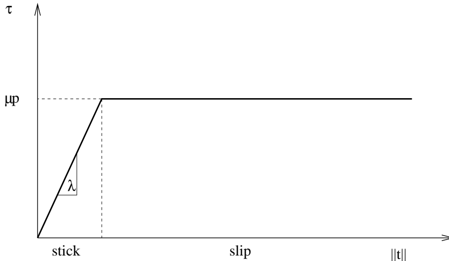
Figure 133: Shear stress versus relative tangential displacement
