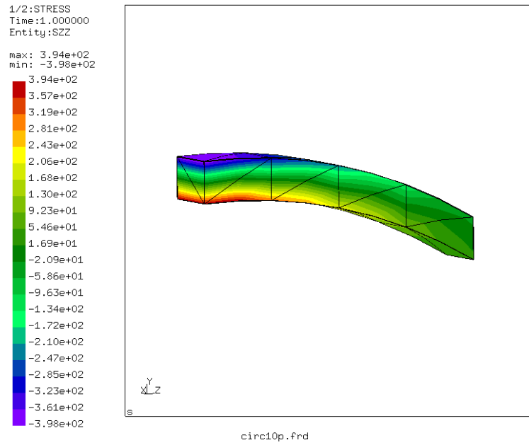
Figure 57: Normal stress in z-direction for the coarse mesh
