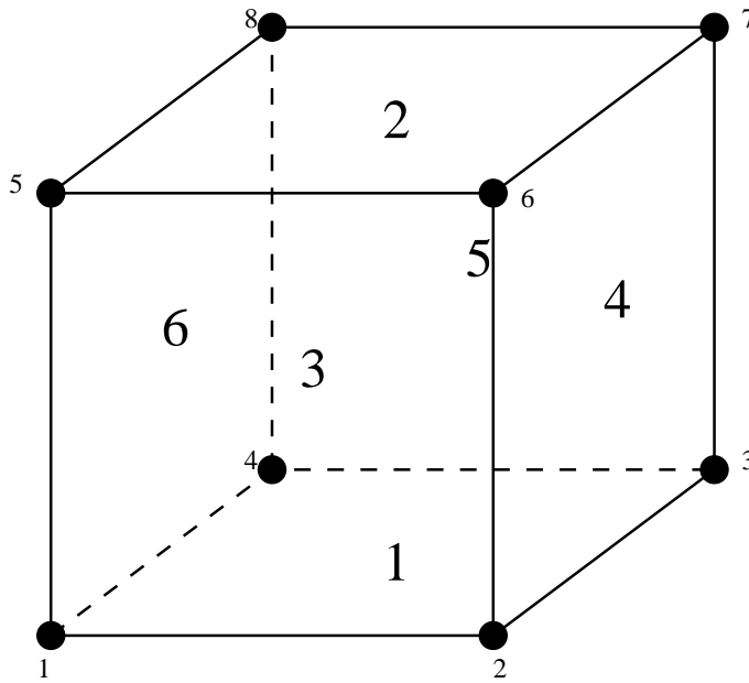
Figure 144: Face numbering for hexahedral elements
