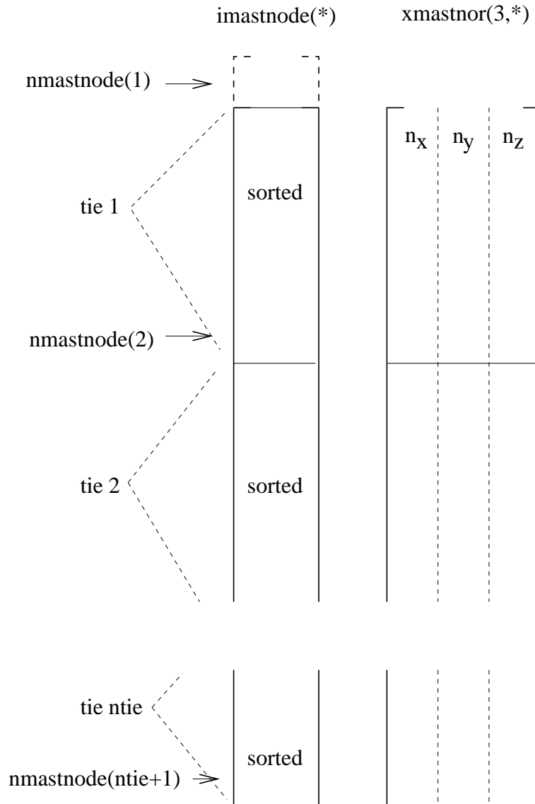
Figure 169: Storage of the master nodes
