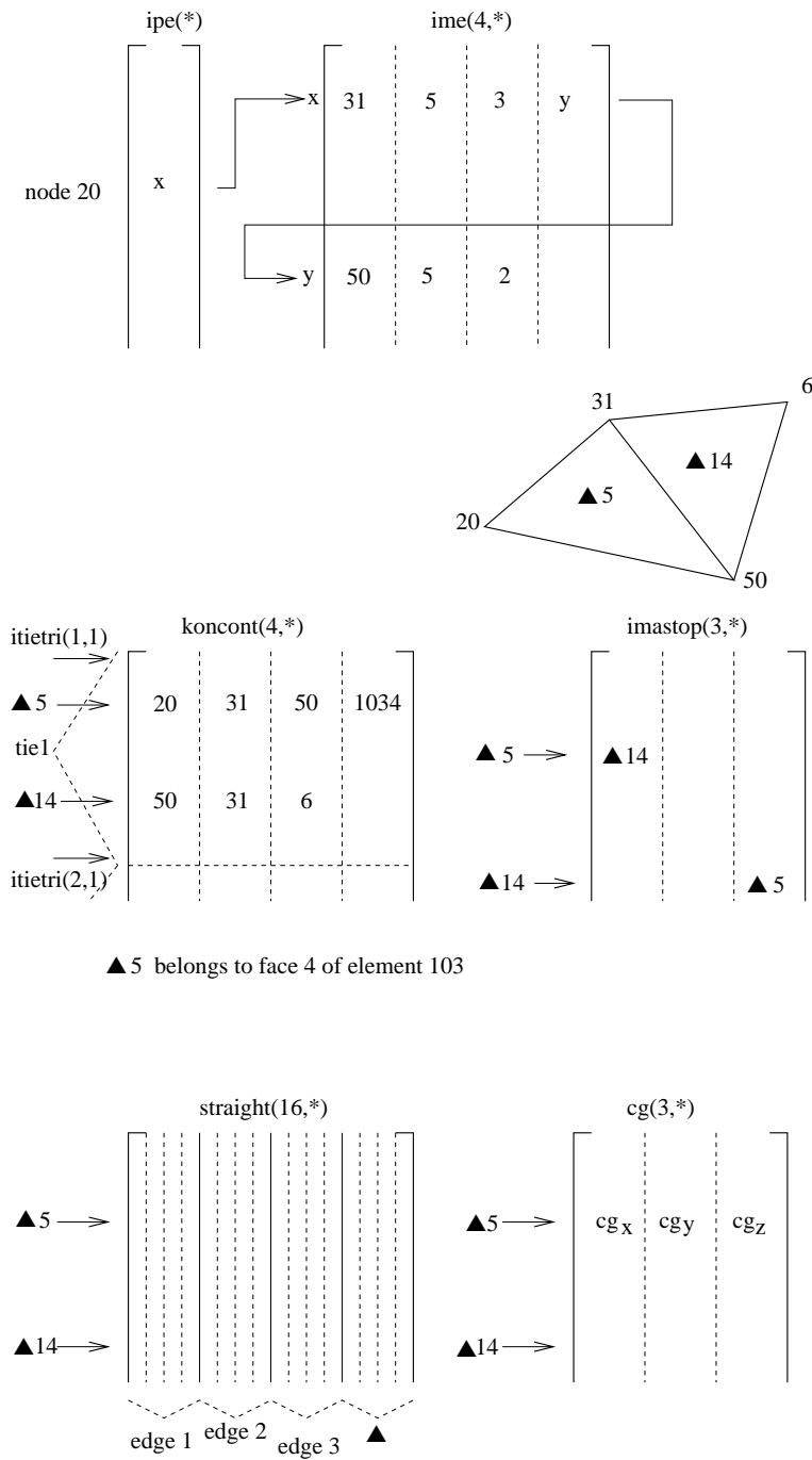
Figure 163: Storage of the triangulation properties
