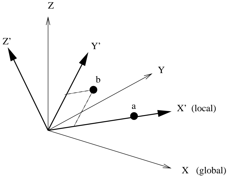
Figure 154: Definition of a rectangular coordinate system
