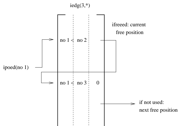
Figure 181: Node per edge relationship
