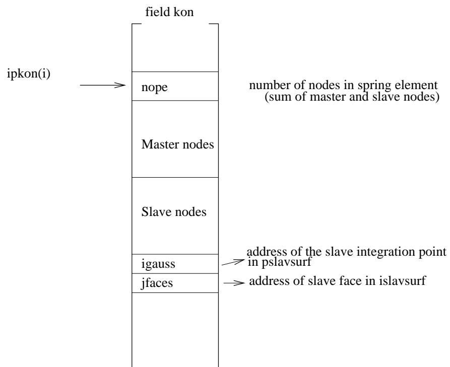
Figure 171: Topology of the face-to-face contact elements
