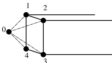
Figure 159: Beam element connection
