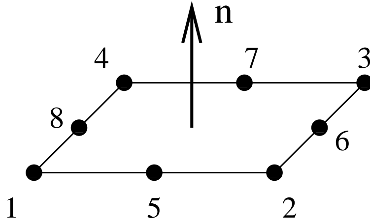
Figure 72: 8-node quadratic element
