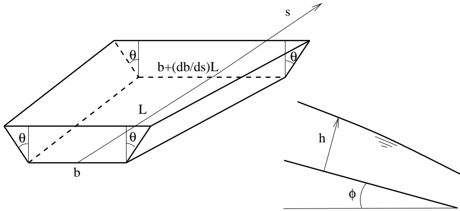
Figure 122: Channel geometry
