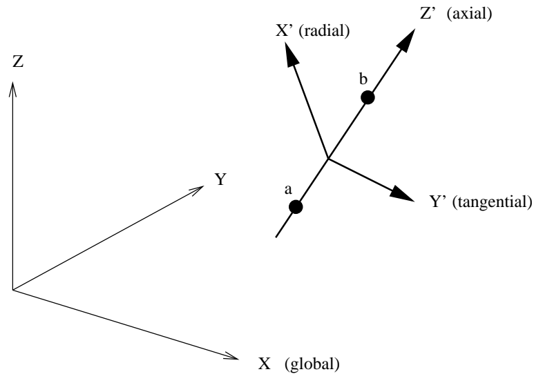
Figure 155: Definition of a cylindrical coordinate system
