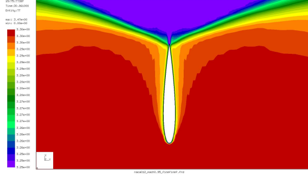
Figure 37: Total temperature
