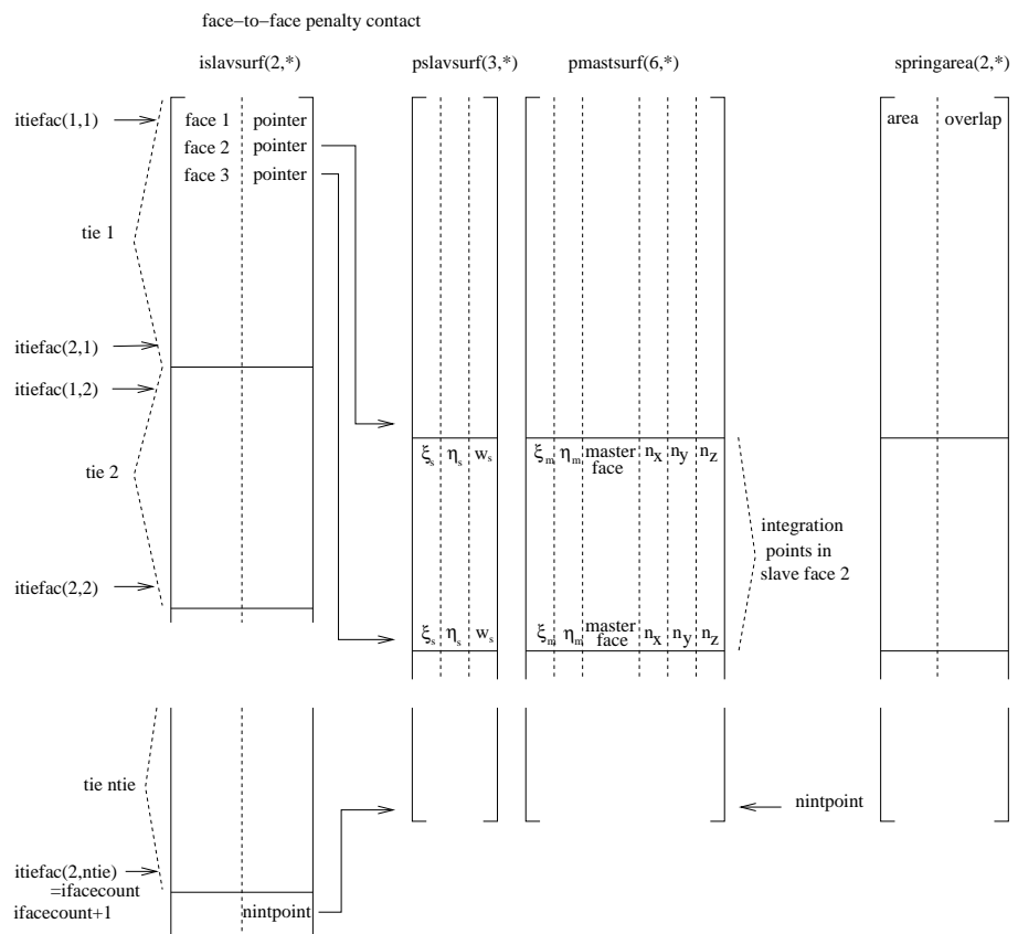
Figure 167: Storage of the slave faces (face-to-face penalty)
