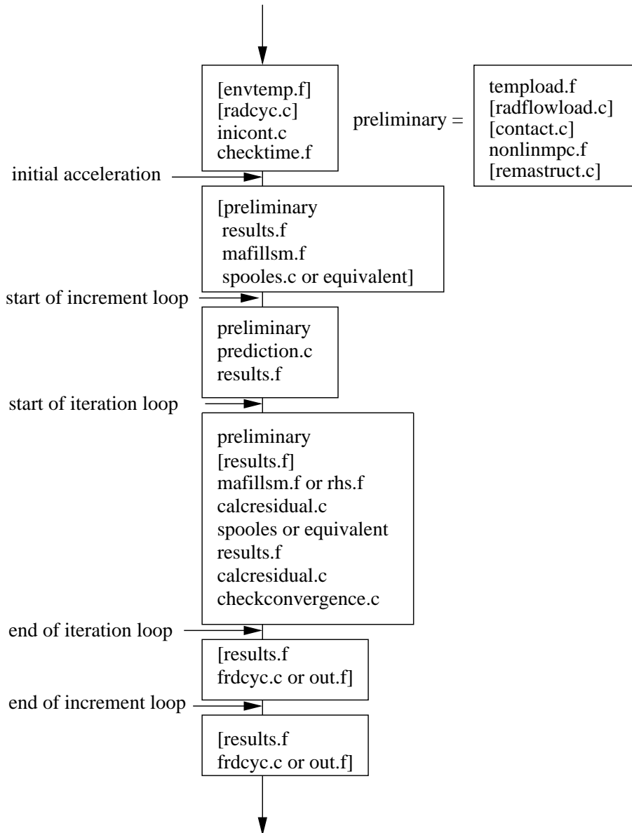
Figure 172: Flow diagram for subroutine nonlingeo
