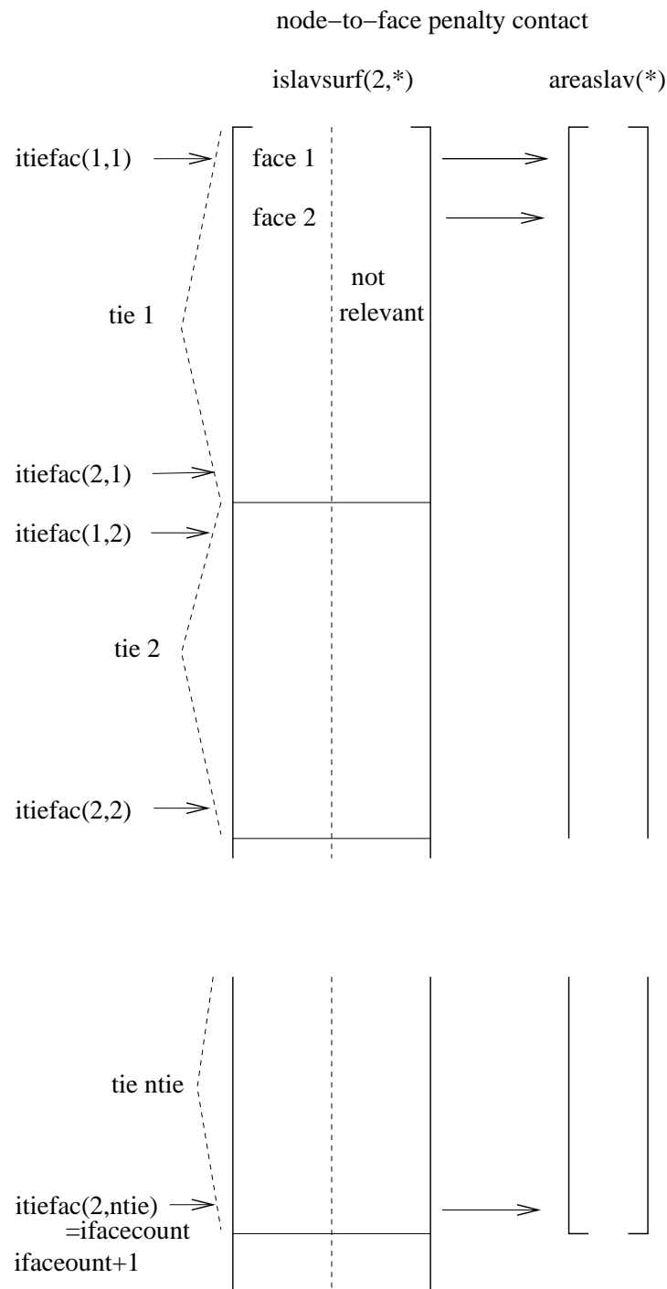
Figure 166: Storage of the slave faces (node-to-face penalty)
