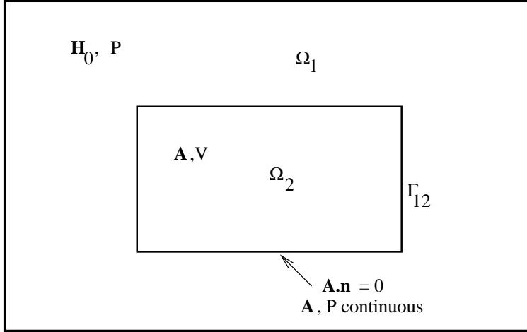
Figure 140: Electromagnetic setup for simply connected bodies
