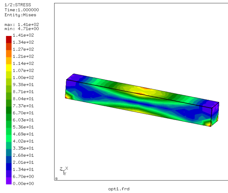
Figure 49: von Mises stress in the starting geometry of the beam
