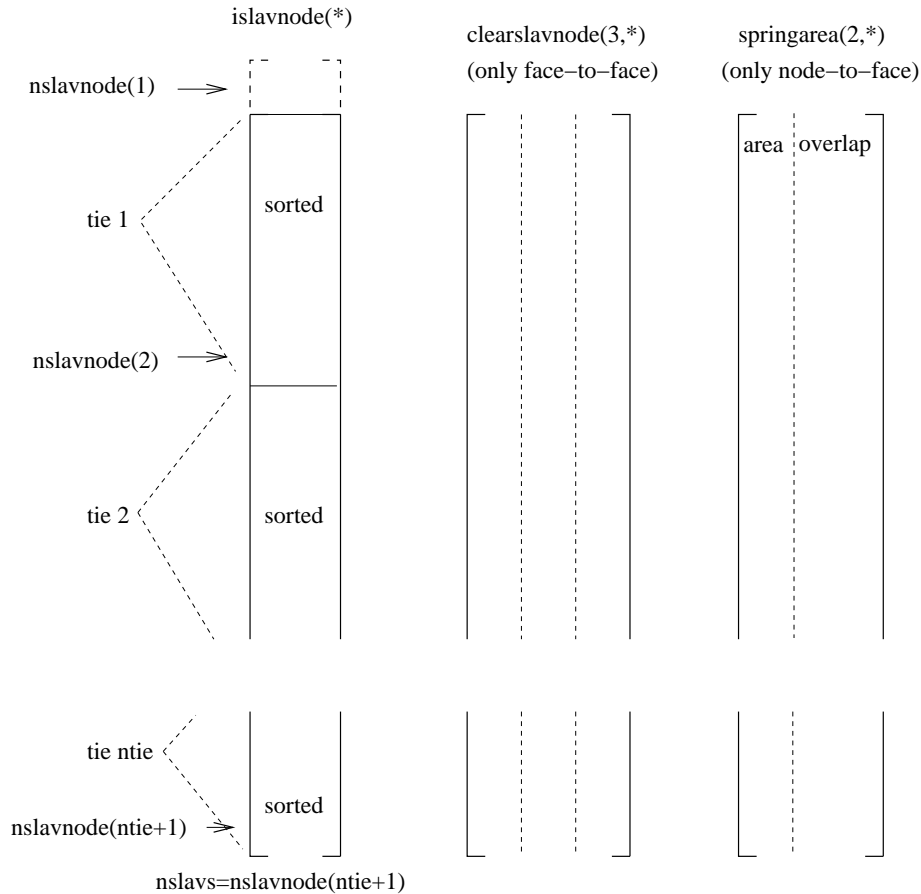
Figure 165: Storage of the slave nodes
