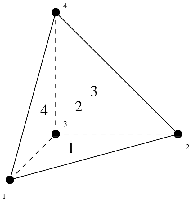
Figure 145: Face numbering for tetrahedral elements
