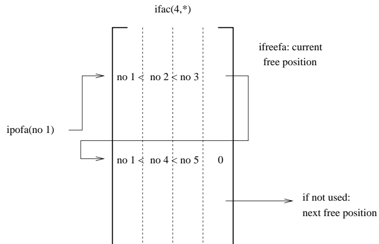
Figure 183: Node per face relationship
