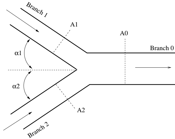
Figure 102: Geometry of a joint fluid section type GE
