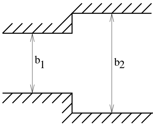
Figure 127: Geometry of an enlargement
