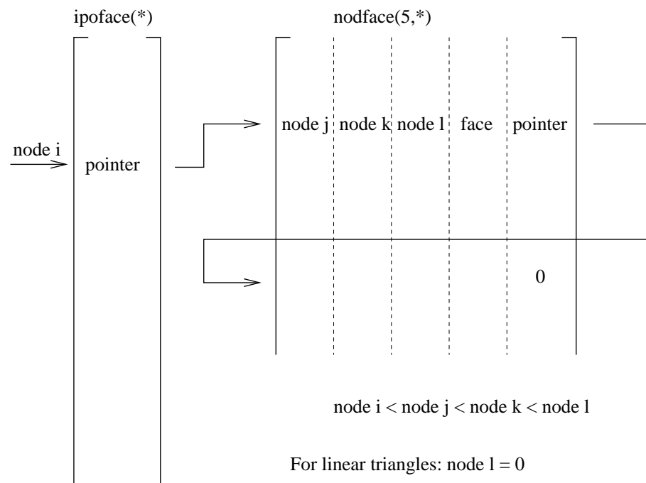
Figure 164: Storage of all faces for the determination of the external faces
