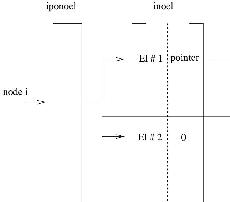
Figure 162: Data structure for all elements belonging to a given node
