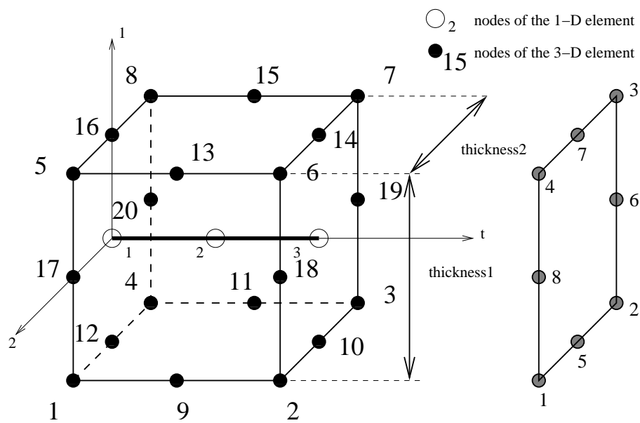
Figure 66: Expansion of a beam element
