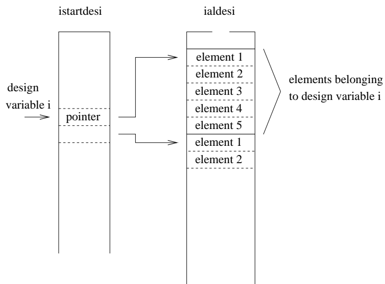
Figure 165: Data structure for all elements belonging to a specific design variable
