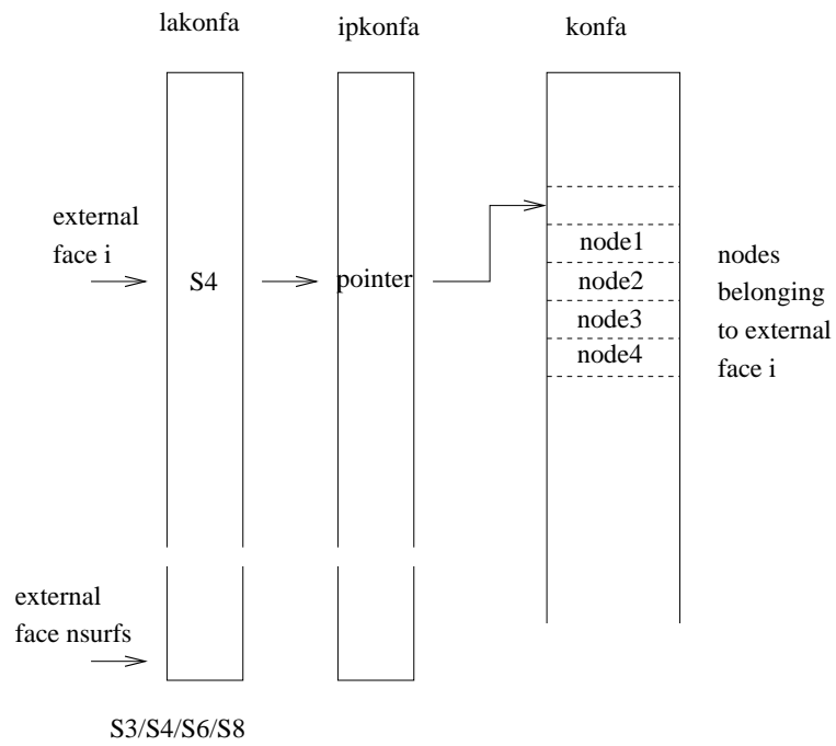
Figure 163: Data structure storing the kind of external face and the nodes belonging to that face
