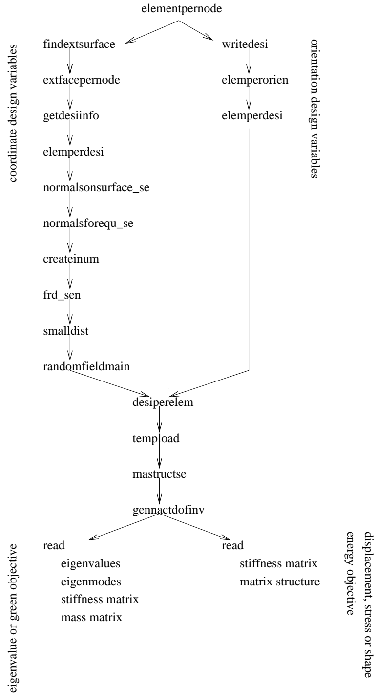
Figure 161: Structure of the preprocessing part
