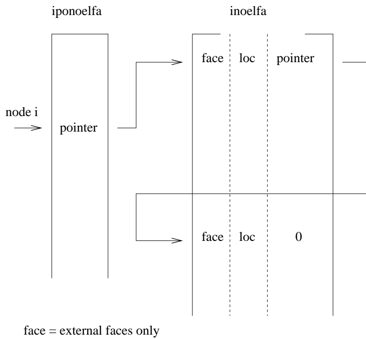
Figure 164: Data structure for all external faces belonging to a given node
