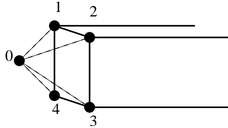
Figure 147: Beam element connection
