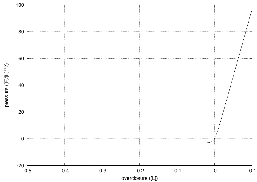
Figure 120: Linear pressure-overclosure relationship
