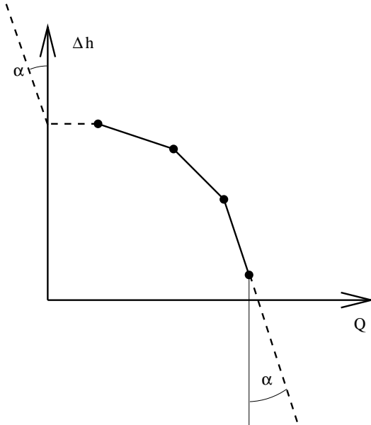
Figure 109: Pump Characteristic
