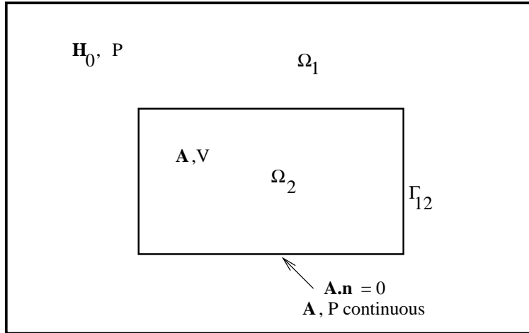
Figure 128: Electromagnetic setup for simply connected bodies
