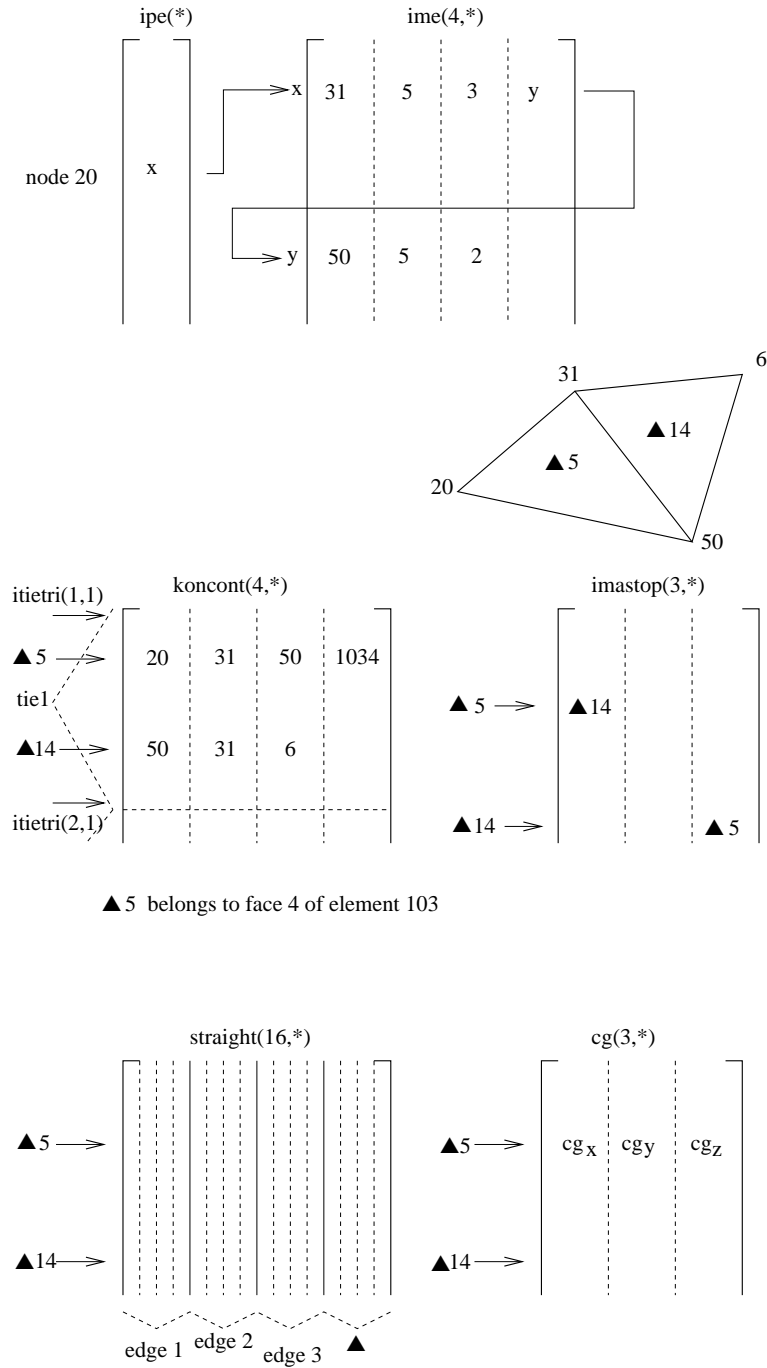
Figure 150: Storage of the triangulation properties
