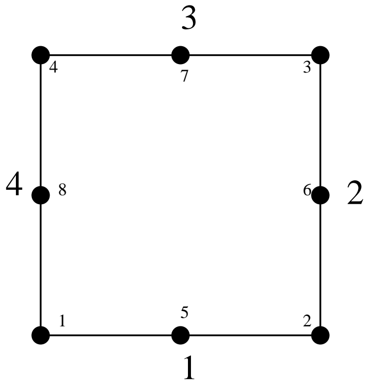
Figure 63: Face numbering for quadrilateral elements
