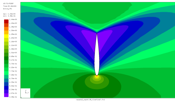
Figure 35: Static pressure
