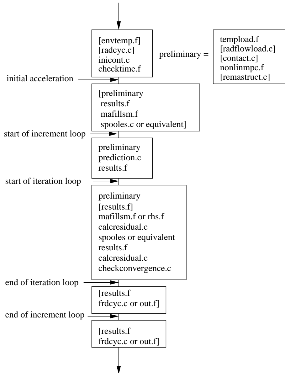
Figure 159: Flow diagram for subroutine nonlinge
