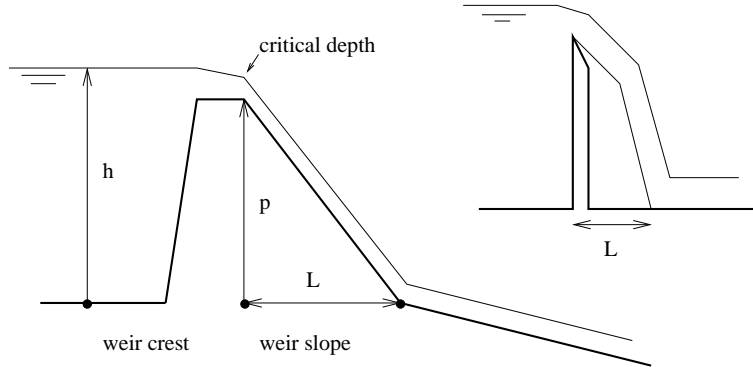
Figure 112: Weir geometry
