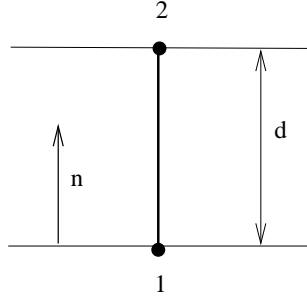
Figure 69: Definition of a GAPUNI element
