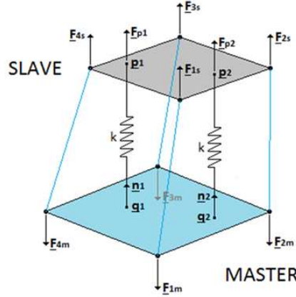
Figure 123: Creation of a face-to-face penalty contact element
