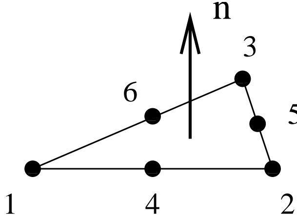
Figure 58: 6-node triangular element
