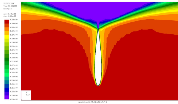
Figure 37: Total temperature
