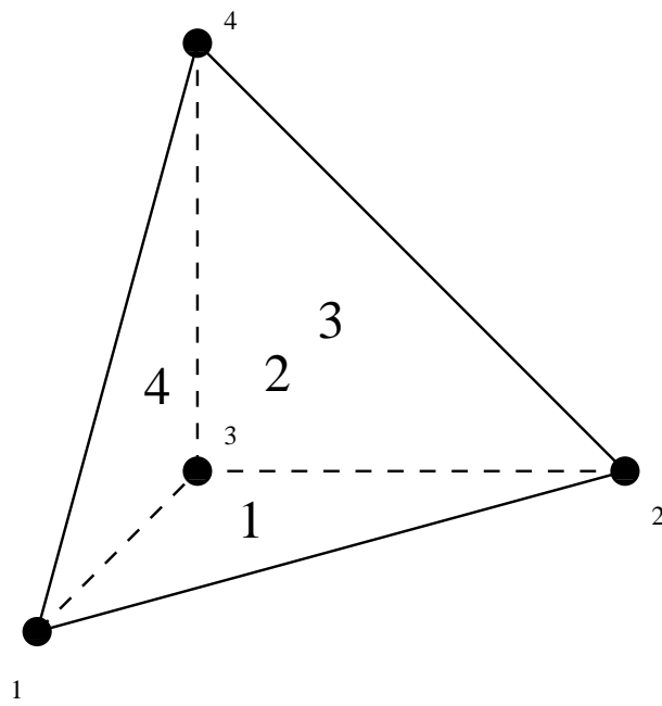
Figure 133: Face numbering for tetrahedral elements
