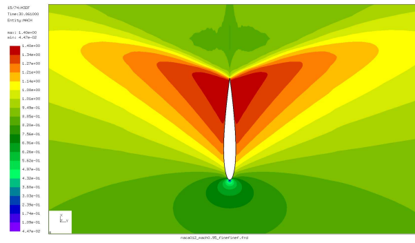
Figure 34: Mach number
