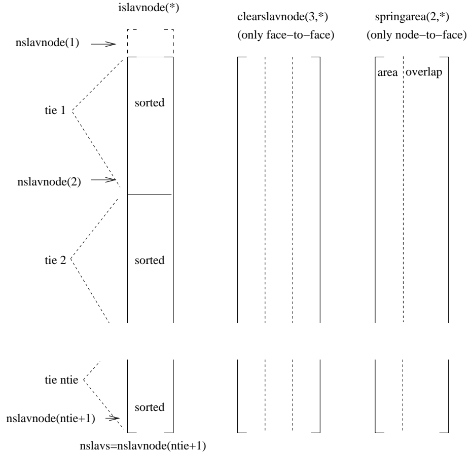
Figure 152: Storage of the slave nodes
