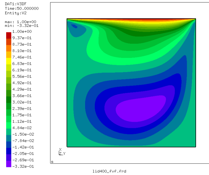
Figure 28: y-component of the velocity in the lid-driven cavity
