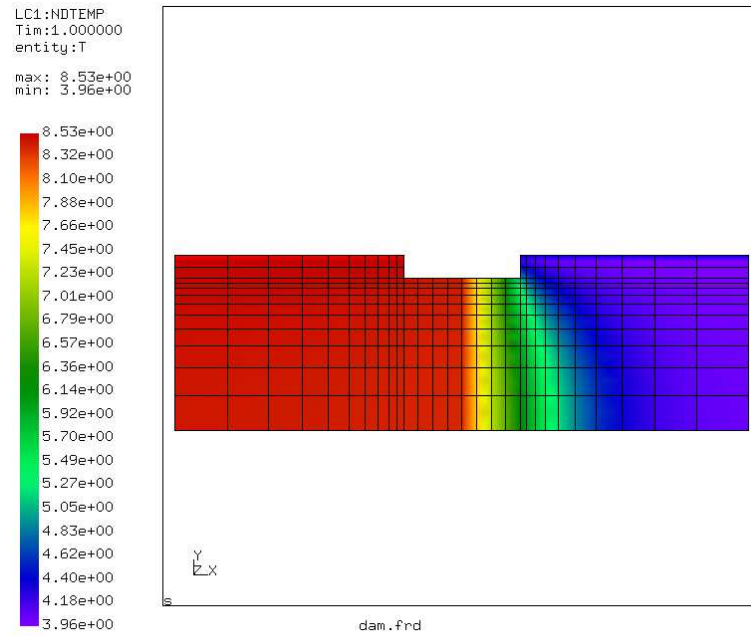
Figure 22: Total head
