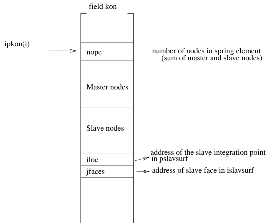
Figure 158: Topology of the face-to-face contact elements
