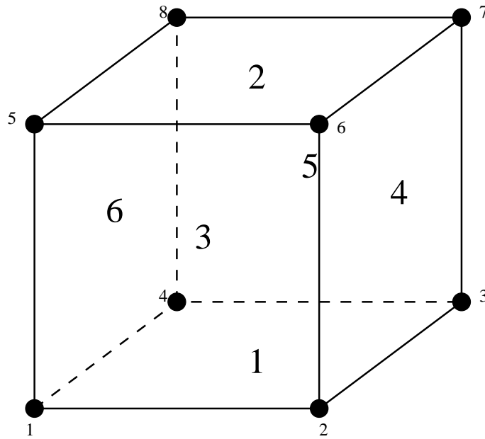
Figure 132: Face numbering for hexahedral elements
