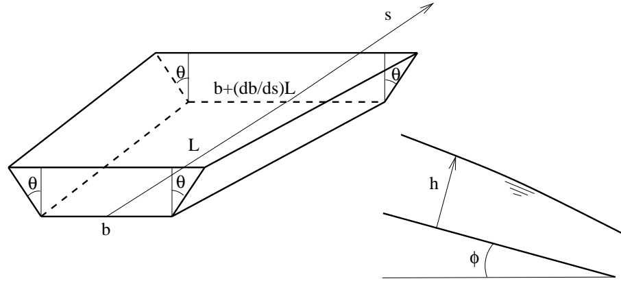
Figure 110: Channel geometry
